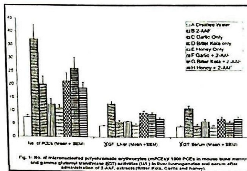
Fig. 1: No. of micronucleated polychromatic erythrocytes (mPCEs)/1000 PCEs in mouse bone marrow and gamma glutamyltransferase (GT) activities (U/L) in liver homogenates and serum after administration of 2-AAF, extracts (bitter kola, garlic and honey).
