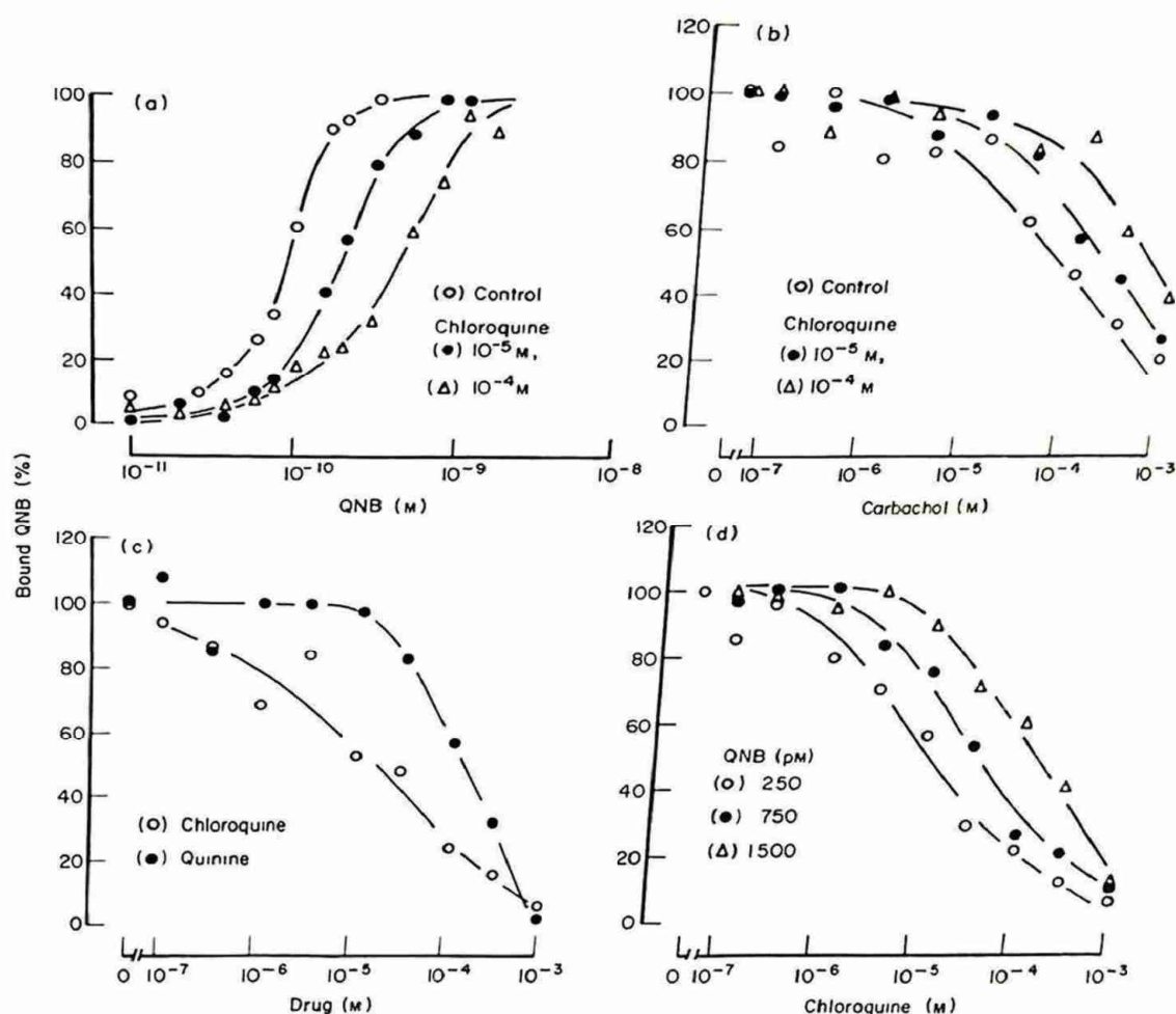
Fig. 1. Binding of chloroquine to muscarinic receptors. (a) Shift of QNB saturation curve by chloroquine. Labelling of muscarinic receptors was done using increasing QNB concentrations in the absence and in the presence of chloroquine. (b) Shift of QNB-carbachol competition curve by chloroquine. Various carbachol concentrations were used to decrease QNB binding, in the absence and in the presence of chloroquine. The QNB concentration used to label the receptors was 750 pM. (c) Inhibition of muscarinic-specific QNB binding with increasing chloroquine or quinine concentrations in the presence of a constant QNB concentration (750 pM). (d) Inhibition of QNB binding with increasing chloroquine concentrations as in (c), but for three different QNB concentrations.
