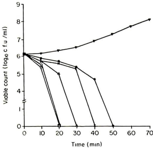
Fig. 2. The effect of HCl on the viable count of Shigella dysenteriae at different pH values: (○) pH 2, (□) pH 3, (△) pH 4, (×) pH 5, (●) pH 6, (▼) pH 7.3.
