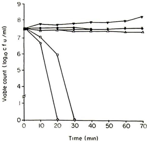
Fig. 5. The effect of HCl on the viable count of Salmonella typhi at different pH values: (○) pH 2, (□) pH 3, (△) pH 4, (×) pH 5, (●) pH 6, (▼) pH 7.3.
