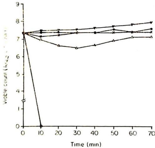
Fig. 3. The effect of HCl on the viable count of Campylobacter jejuni at different pH values: (○) pH 2, (□) pH 3, (△) pH 4, (×) pH 5, (●) pH 6, (▼) pH 7.3.
