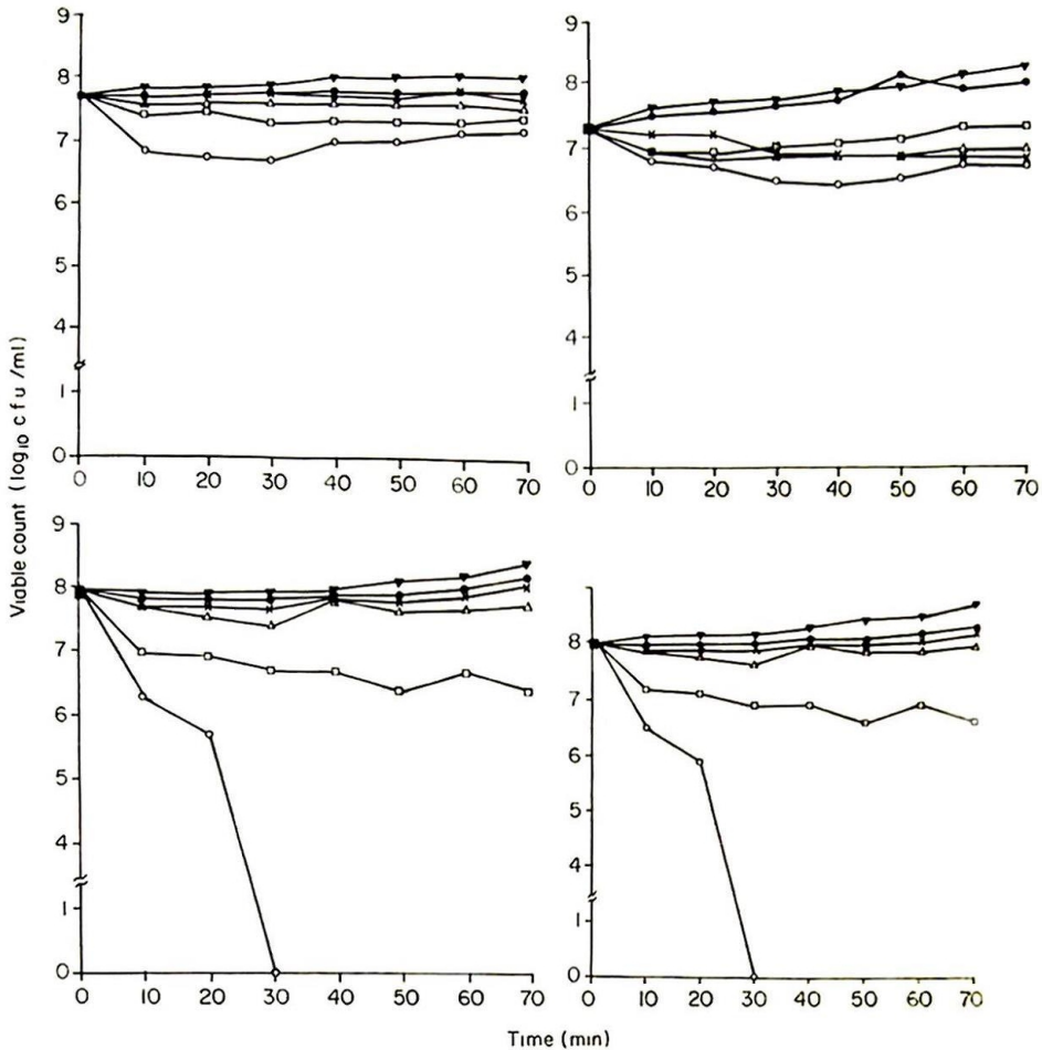
Fig. 1. The effect of HCl on the viable count of (a) E. coli , (b) enteropathogenic E. coli , (c) enteroinvasive E. coli and (d) enterotoxigenic E. coli at different pH values: (O) pH 2, (□) pH 3, (△) pH 4, (×) pH 5, (●) pH 6, (▼) pH 7.3.
